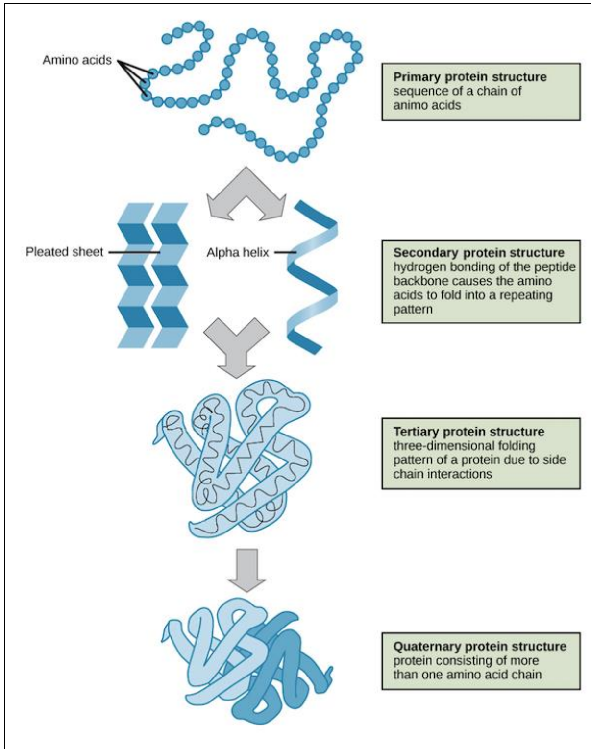
Figure (2) The order of protein structure
